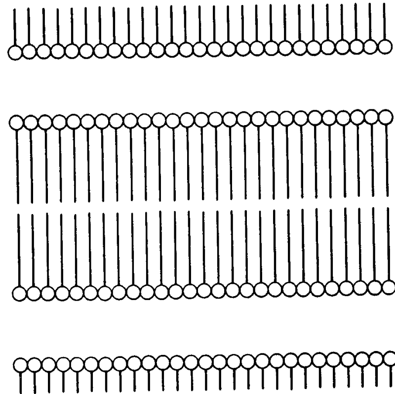
The McBain lamellar micelle
